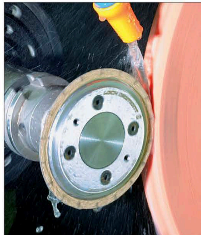
drebojet®-PLUS during path-controlled dressing of a grinding wheel
