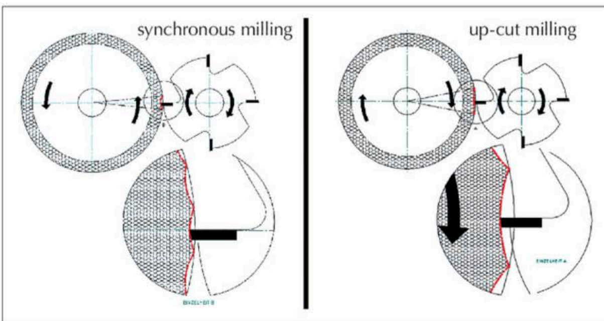
Schematic diagram: development of the different commas during dressing in synchronous milling and up-cut milling
