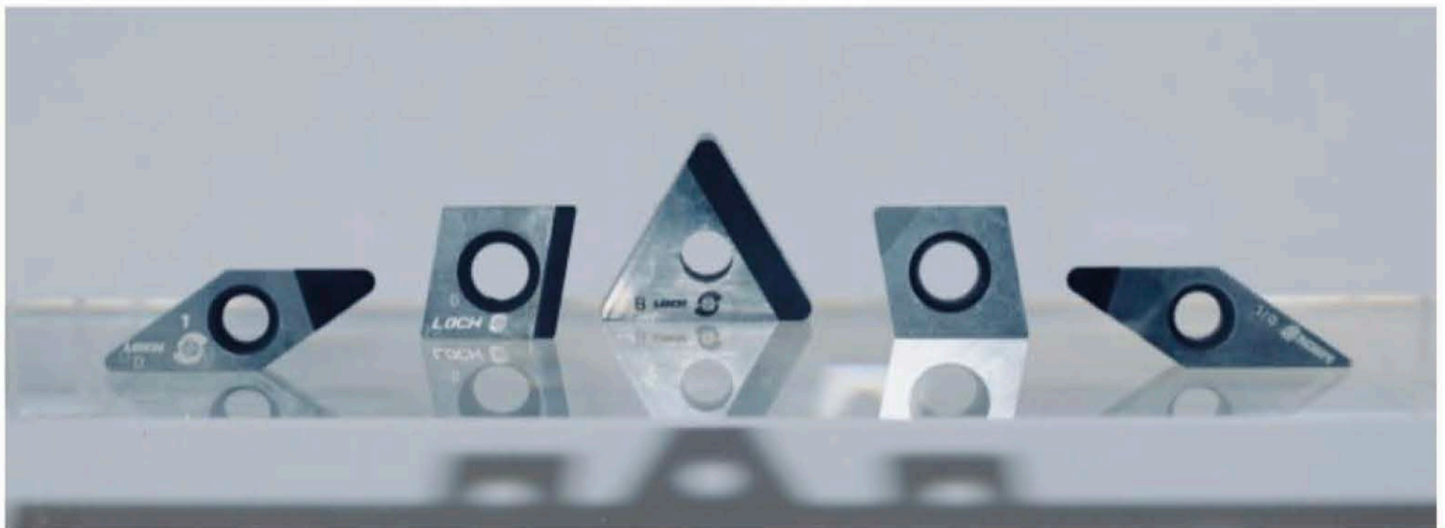
A selection of PCD and PCBN inserts, developed during the 1970s, for milling and turning.
