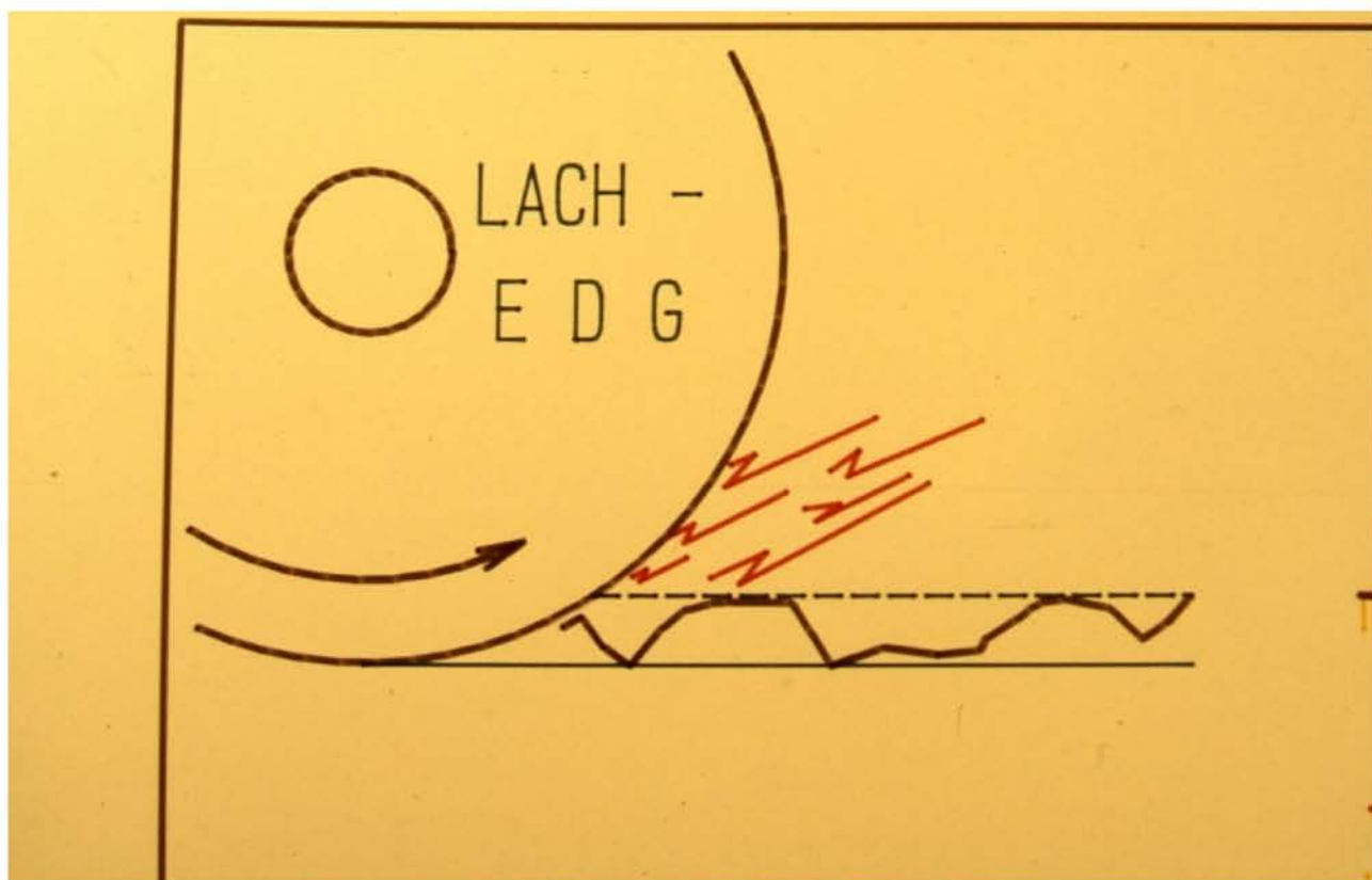
A diagram of spark erosion grinding with rotating electrode, either graphite or copper.
